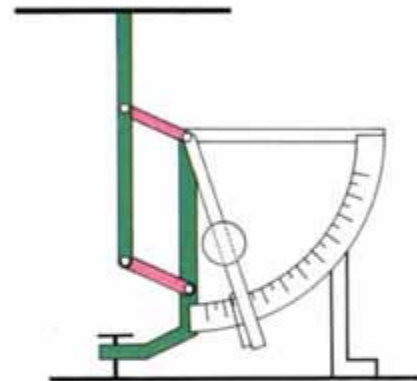
28.2 Briefwaage
