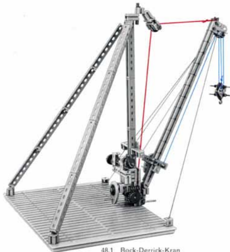
48.1 Bock-Derrick-Kran
