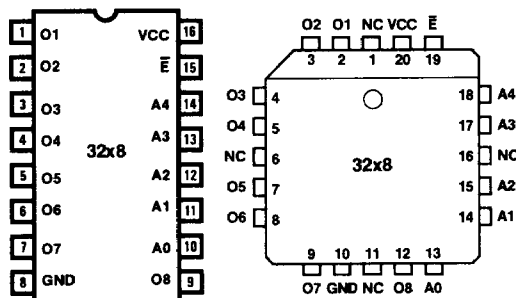
Plastic Chip Carrier
