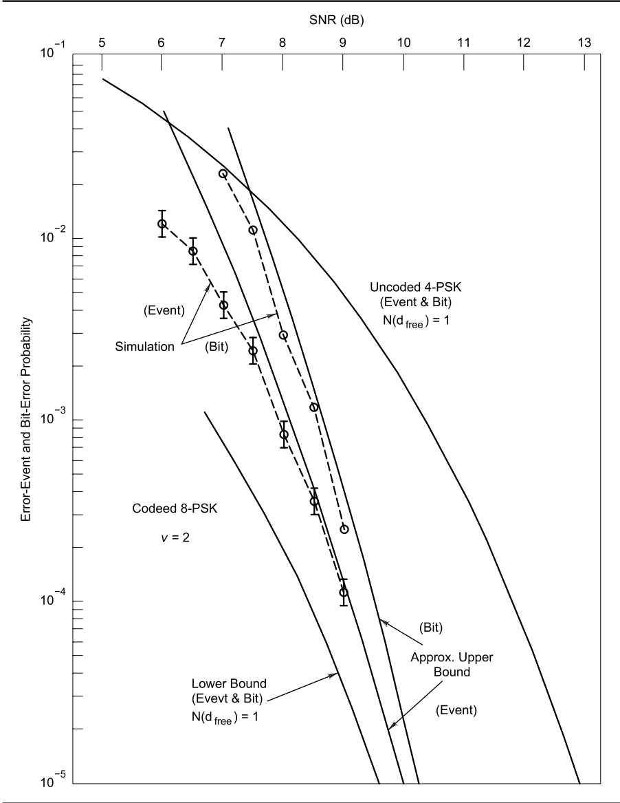
Fig 9—TC8PSK vs. QPSK
