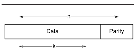
Fig 15—RS(n,k) Encoded Block
