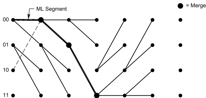
Fig 8—Viterbi Decoding
