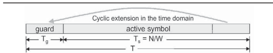
Fig 3—Guard Band
