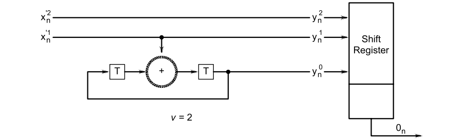
Fig 6—Convolutional Coding
