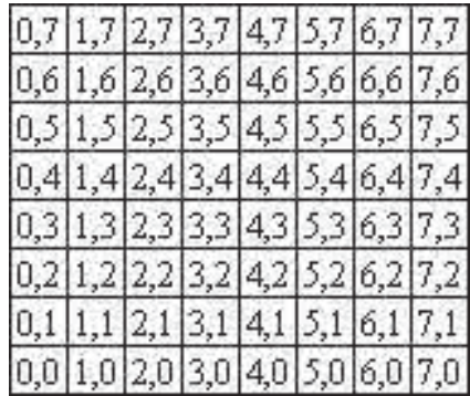
Fig 10—64QAM Signal Constellation with Coded I and Q Tribits shown in Octal
