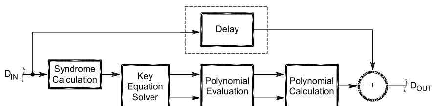
Fig 16—RS Error Correction Process
